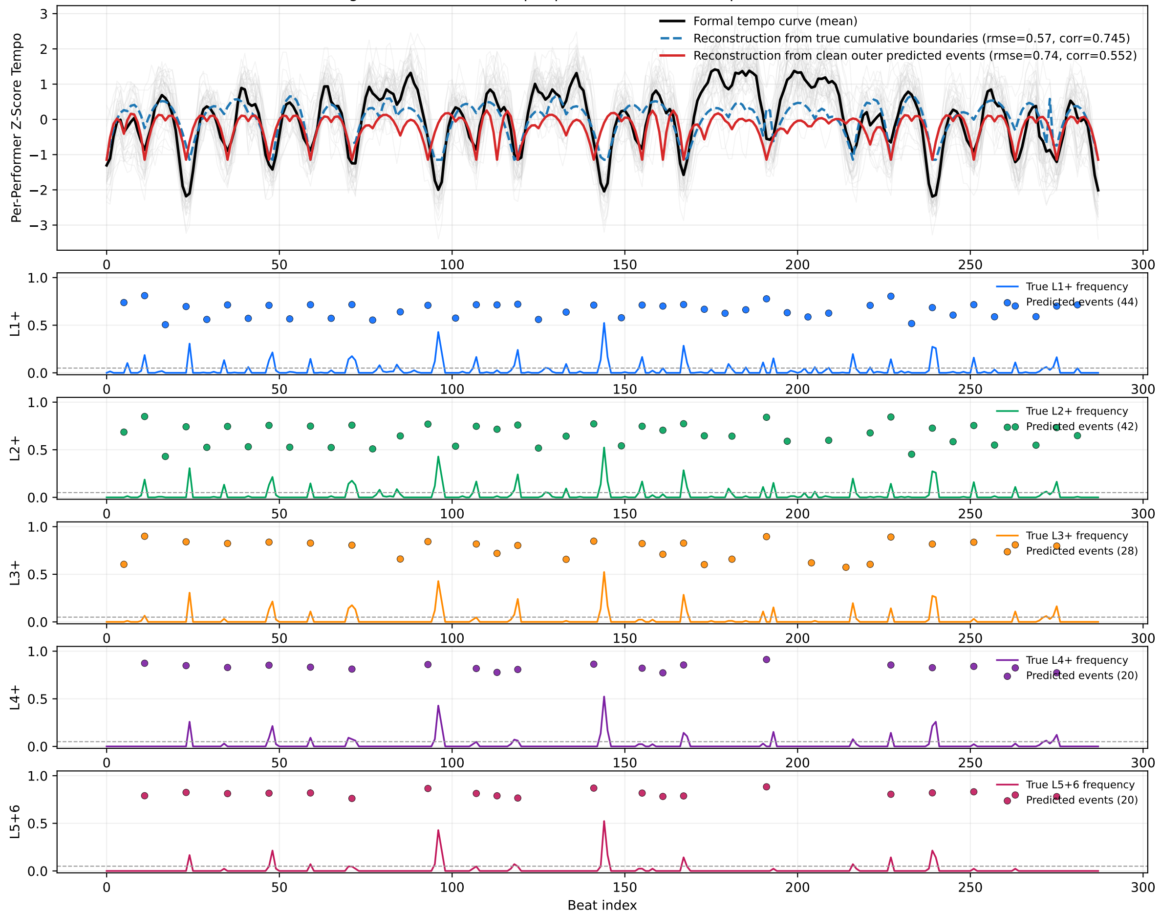
M06-2: merged L5+6 clean outer per-performer z-score tempo reconstruction (seed 44)
